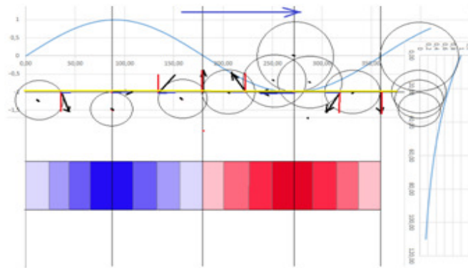
Figure 7. Scheme for the propagation of vertical forces on the ASRBHK turbine SB.
