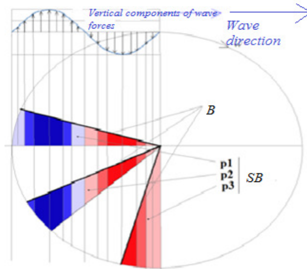
Figure 7. Scheme for the propagation of vertical forces on the ASRBHK turbine SB.
