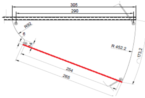
Figure 6. Self-regulated blade of turbine (SB).
