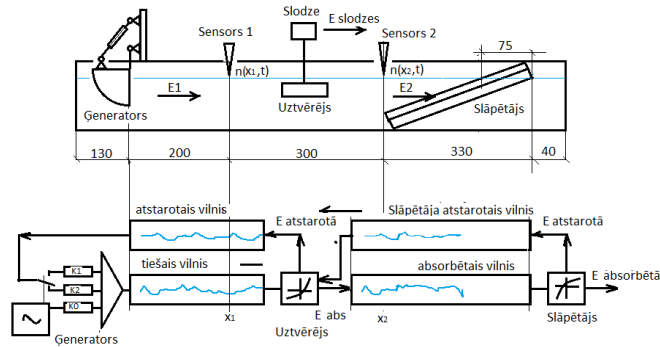
Fig.4. Wave Process Analysis Scheme, [15].
