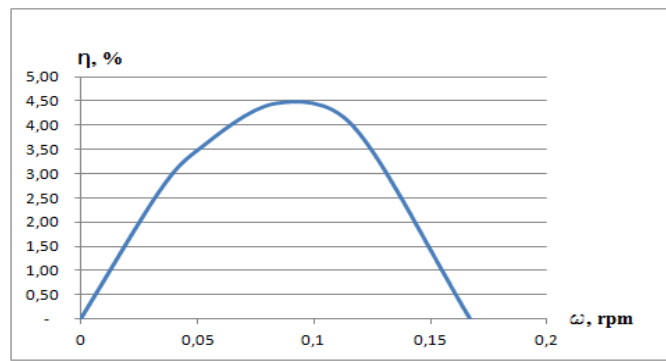
Figure 5. Mechanically tensioned ASRBHK turbine efficiency coefficient curve.
